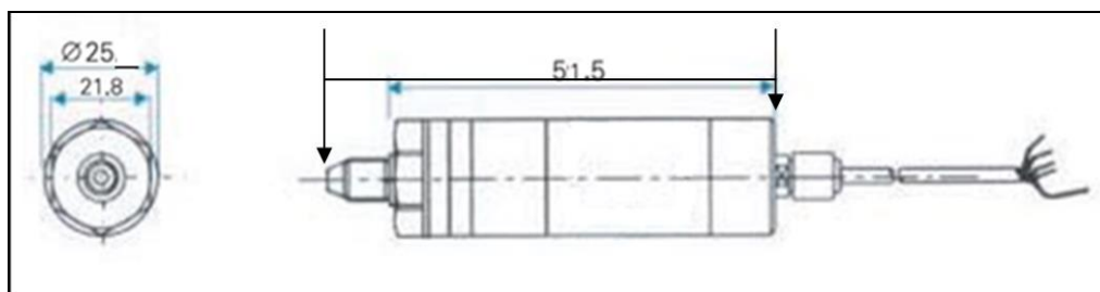
Drawing 1 Dimensions
